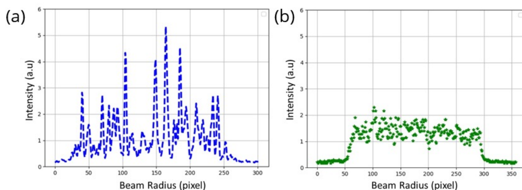
Figure 3: Laser beam profile at the entrance of the optical fiber (a) before beam shaping (b) after beam
