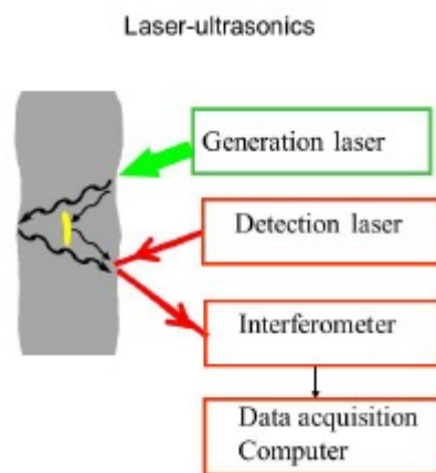
Figure 1 : Laser ultrasonics apparatus [1]
