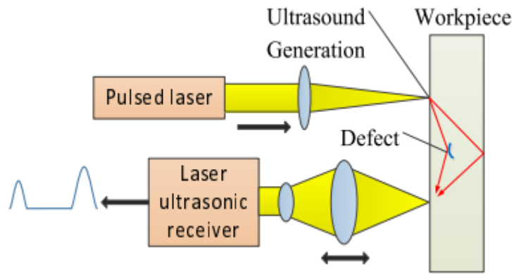
Figure 2 : Laser ultrasonic crack detection principle [2]
