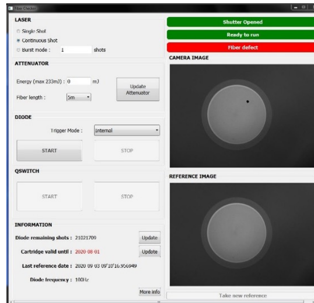
Figure 4 : Optical fiber entrance facet live monitoring after beam shaping
