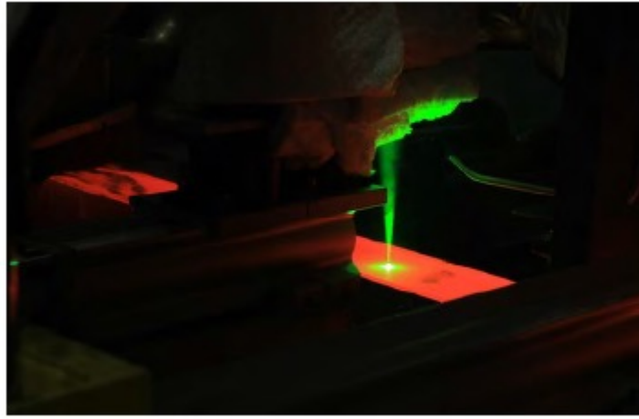
Figure 7 : Optical head located above the steel
